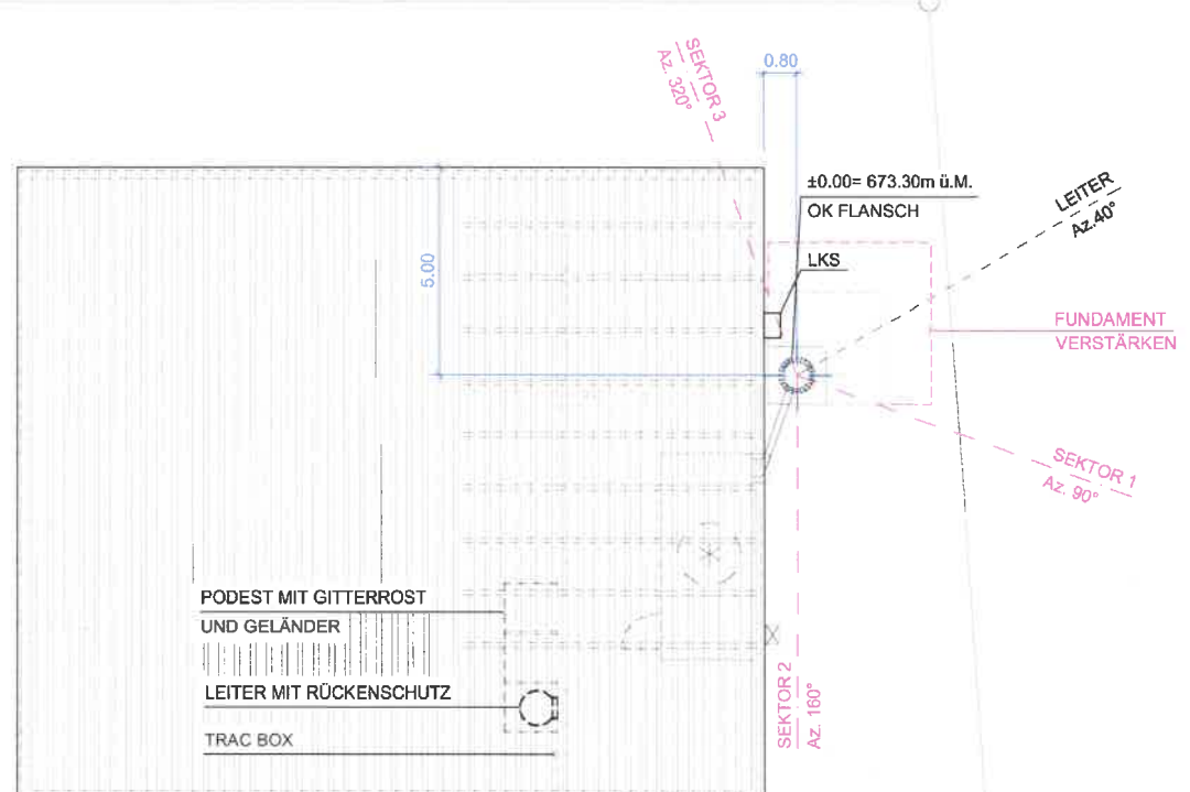
SITUATION 1:200
